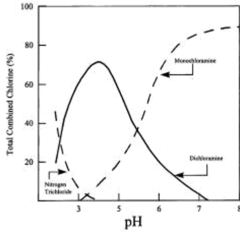
Figure 6-2. Distribution Diagram for Chloramine Species with pH
